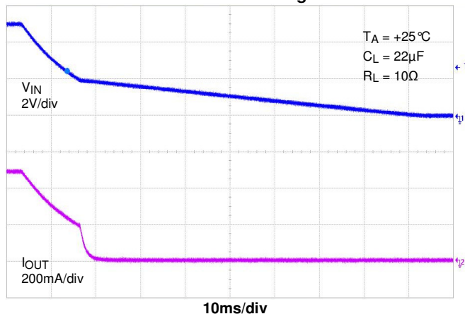
UVLO Decreasing
