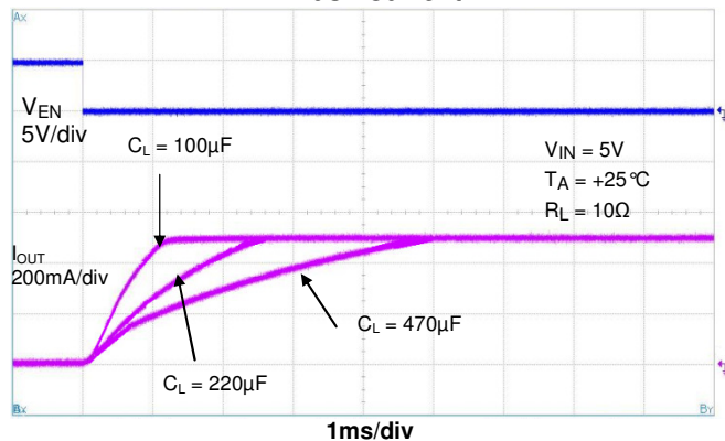
Inrush Current
