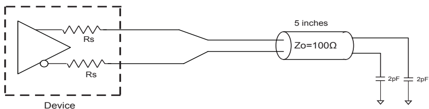
Low-Power HCSL Differential Output Test Load
