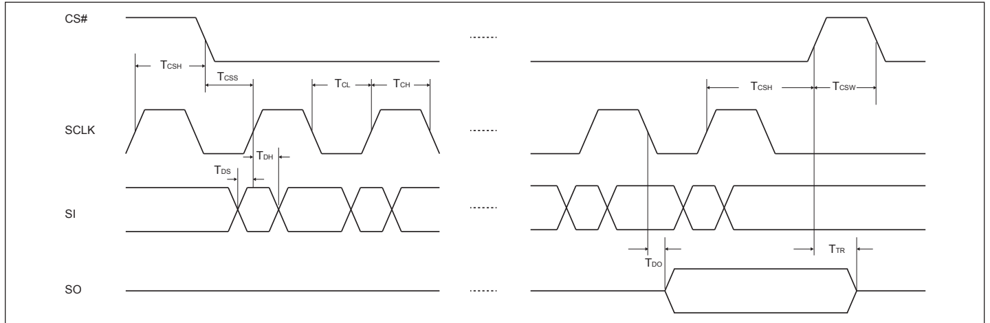
Figure 26. SPI-Bus Timing
