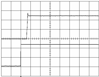
Start-up enabled by connecting V_i at: T_{ref} = +25^{\circ}\text{C} , I_O = 6\text{ A} resistive load, V_i = 12\text{ V} . Top trace: output voltage (0.5 V/div). Bottom trace: input voltage (5 V/div). Time scale: 20 ms/div.
