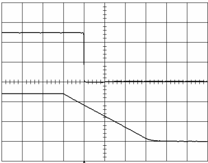
Shut-down enabled by disconnecting V_i at: T_{ref} = +25^{\circ}\text{C} , I_O = 6\text{ A} resistive load, V_i = 12\text{ V} . Top trace: output voltage (0.5 V/div). Bottom trace: input voltage (5 V/div). Time scale: 20 ms/div.
