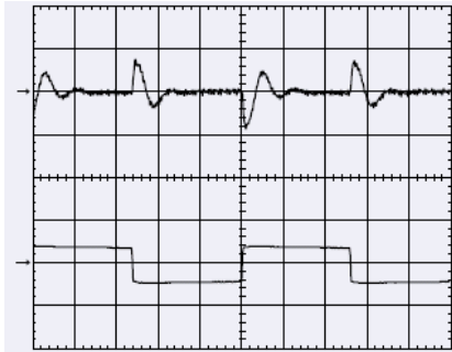
Output voltage response to load current step- change (-2A-2A) at: T_{ref} = +25^{\circ}\text{C} , V_i = 12\text{ V} . Top trace: V_{out}-V_{trk} (50mV/div). Bottom trace: load current (5 A/div). Time scale: 0.1 ms/div.
