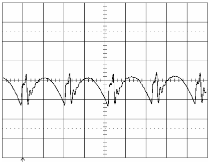
Output voltage ripple (20mV/div) at: T_{ref} = +25^{\circ}\text{C} , I_O = 6\text{ A} resistive load, V_i = 12\text{ V} . Time scale: 2 \mu\text{s} /div See the filter in the Output ripple and noise section (EMC Specification).
