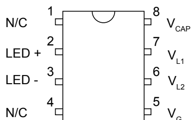
CPC1580P Pinout
