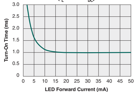
Typical Turn-On Time vs. LED Forward Current ( I_L=130\text{mA}_{DC} )
