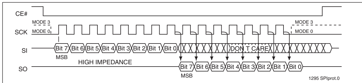
FIGURE 4-1: SPI PROTOCOL
