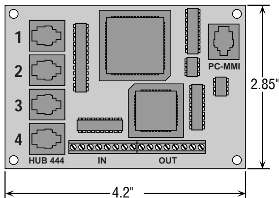
MECHANICAL OUTLINE:
