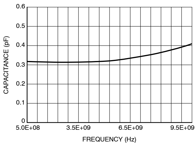
Figure 10. Junction Capacitance; V_R = 0 V, f = 500 MHz – 10 GHz
