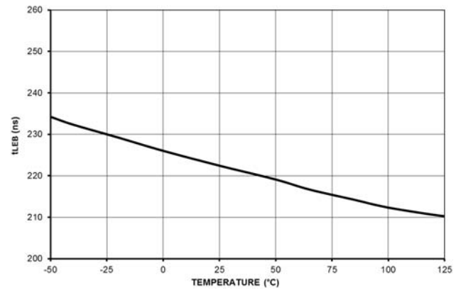
Figure 14. Leading Edge Blanking Duration t LEB
