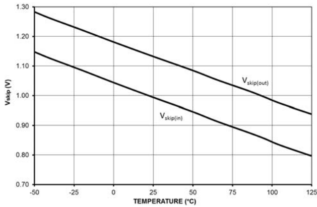
Figure 17. FB Pin Skip-In and Skip-Out Levels V_{skip(in)} and V_{skip(out)}
