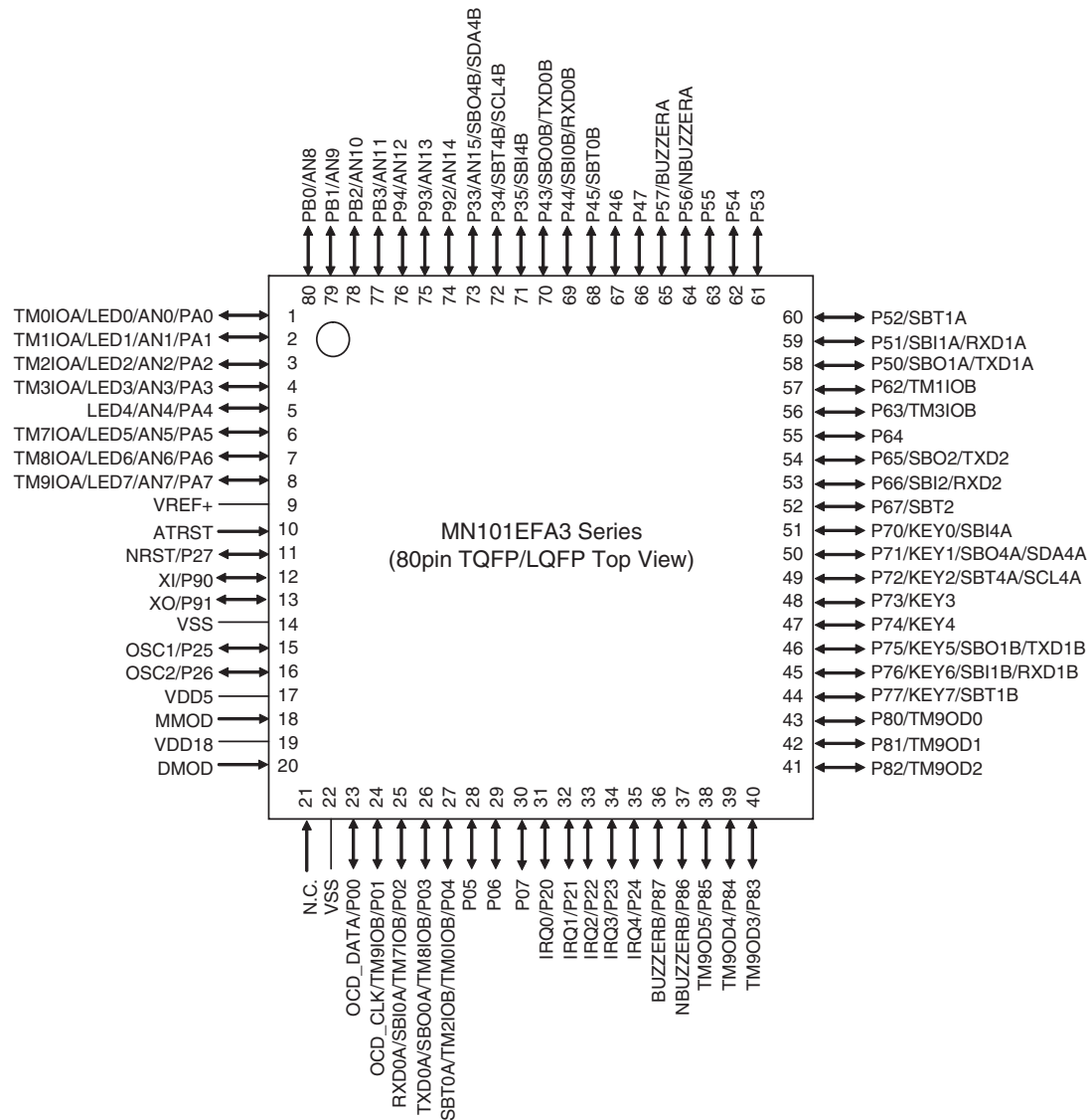
Figure:1.3.3 Pin Configuration (MN101EFA3 Series 80-pin TQFP/LQFP)
