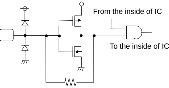
Fig.113 BU3071HFV
