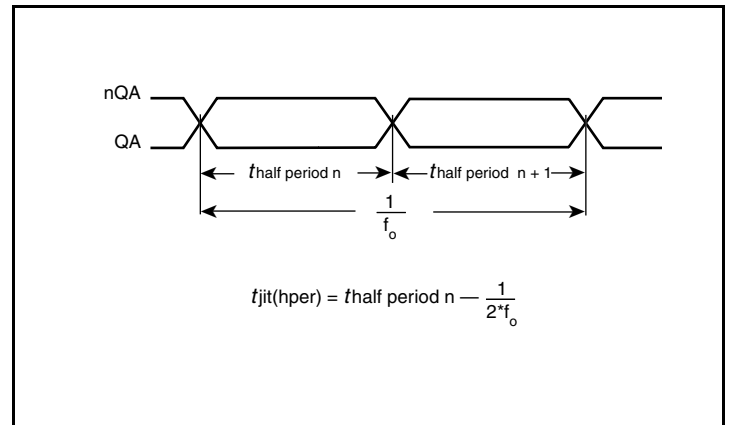
Half Period Jitter
