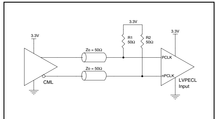
Figure 2D. PCLK/nPCLK Input Driven by a CML Driver
