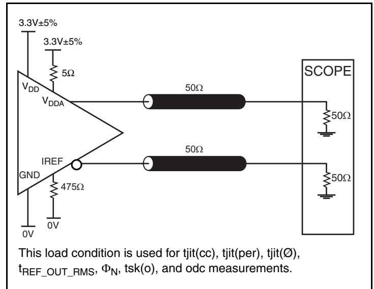
3.3V HCSL Output Load Test Circuit 2
