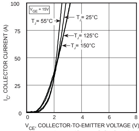
FIGURE 1, Output Characteristics ( T_J = 25^\circ C )
