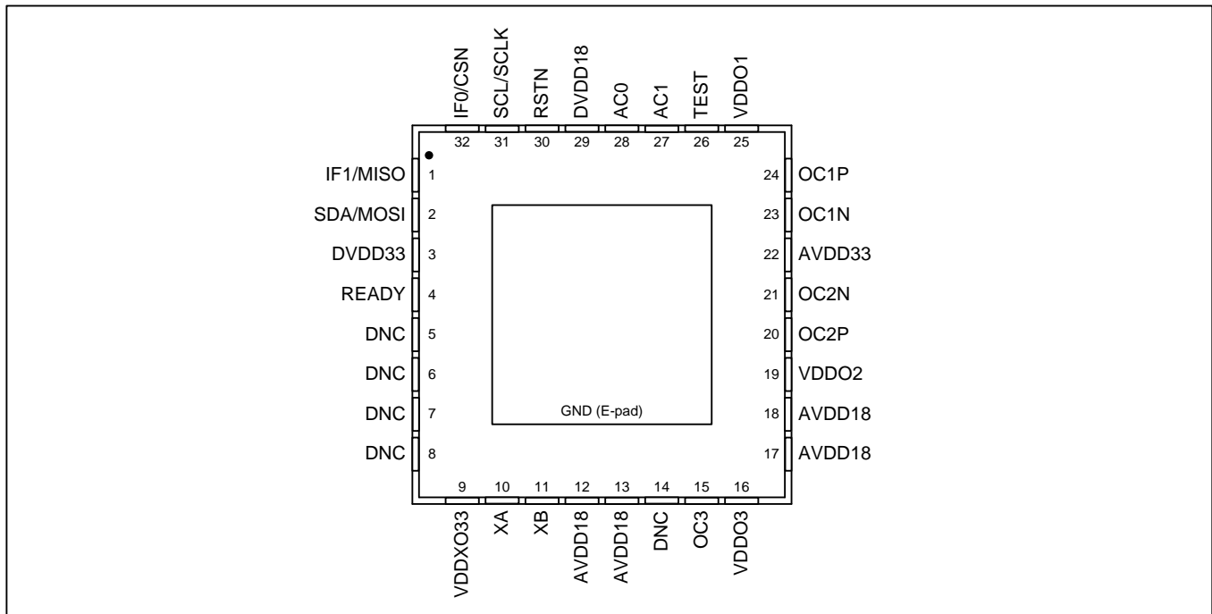
Figure 2 - Pin Diagram
