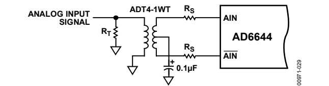
Figure 29. Transformer-Coupled Analog Input Circuit
