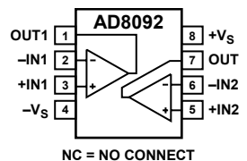
NC = NO CONNECT Figure 3. MSOP-8 and SOIC-8 (RM-8, R-8)
