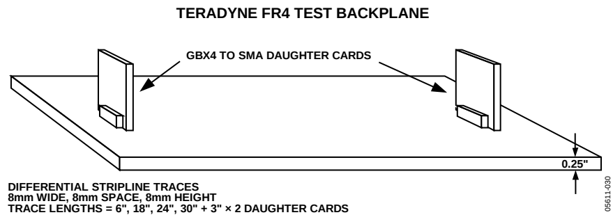
Figure 30. Test Backplane
