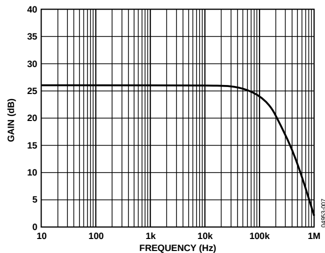
Figure 7. Typical Small Signal Bandwidth ( V_{OUT} = 200 mV p-p)
