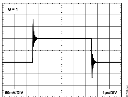
Figure 35. Small Signal Response ( G = 1 ), R_L = 10 kΩ, C_L = 100 pF
