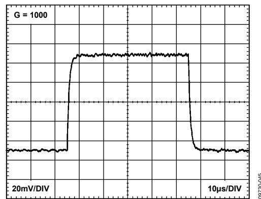
Figure 38. Small Signal Response ( G = 1000 ), R_L = 10 kΩ, C_L = 100 pF
