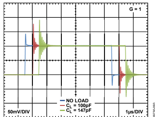
Figure 39. Small Signal Response with Various Capacitive Loads ( G = 1 ), R_L = \text{Infinity}
