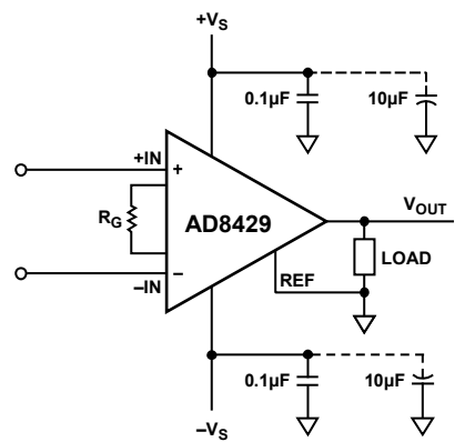
Figure 49. Supply Decoupling, REF, and Output Referred to Local Ground
