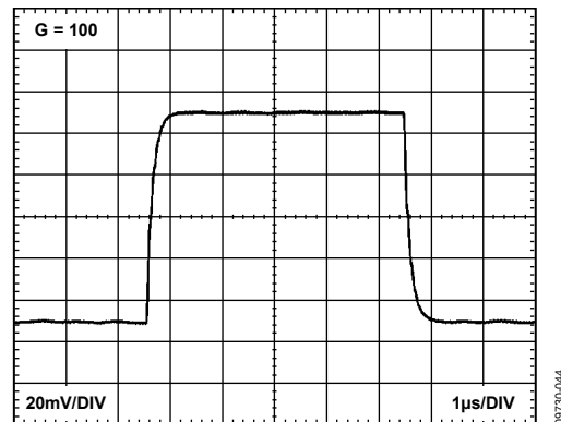
Figure 37. Small Signal Response ( G = 100 ), R_L = 10 kΩ, C_L = 100 pF
