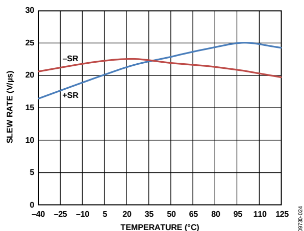
Figure 17. Slew Rate vs. Temperature, V_S = \pm 15 V ( G = 1 )
