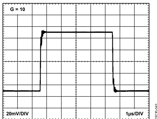
Figure 36. Small Signal Response ( G = 10 ), R_L = 10 kΩ, C_L = 100 pF
