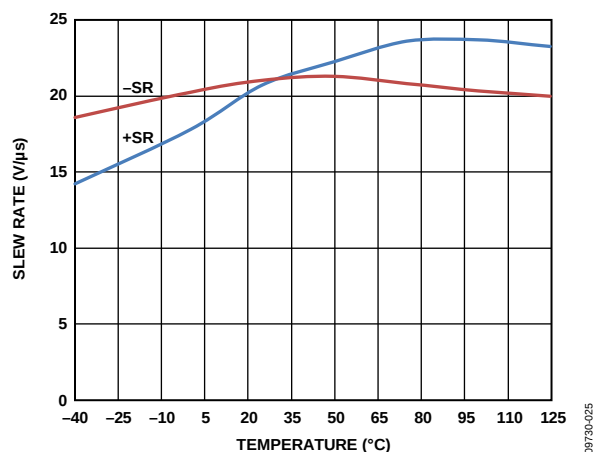
Figure 18. Slew Rate vs. Temperature, V_S = \pm 5 V ( G = 1 )
