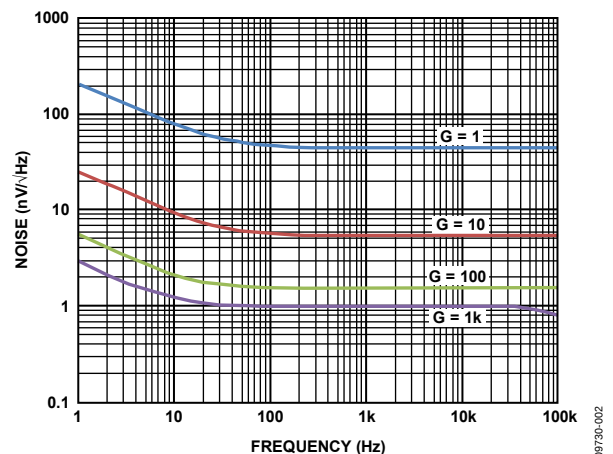
Figure 2. RTI Voltage Noise Spectral Density vs. Frequency
