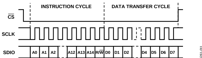
Figure 46. Serial Register Interface Timing, LSB First, Register 0x000, Bit 6 and Bit 1 = 1
