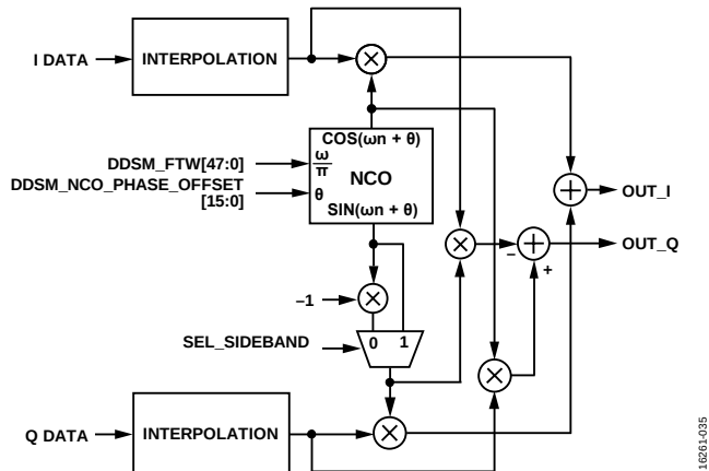
Figure 72. NCO Modulator Block Diagram
