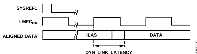
Figure 64. DYN_LINK_LATENCY_x Illustration
