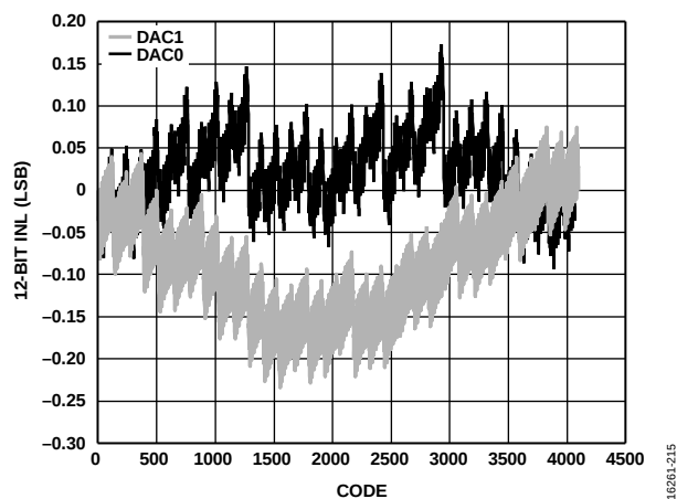
Figure 41. INL, I_{OUTFS} = 20 mA, 12-Bit Resolution
