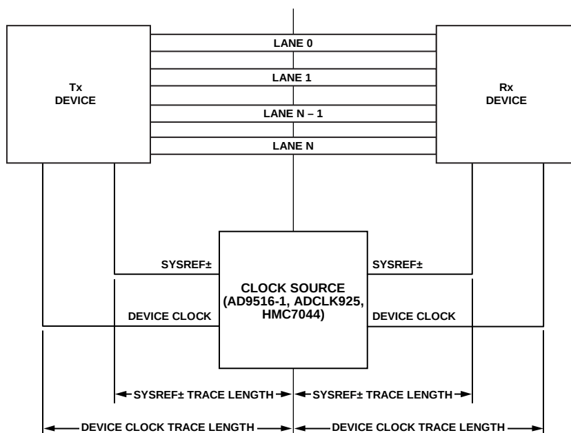
Figure 86. SYSREF \pm Signal and Device Clock Trace Length
