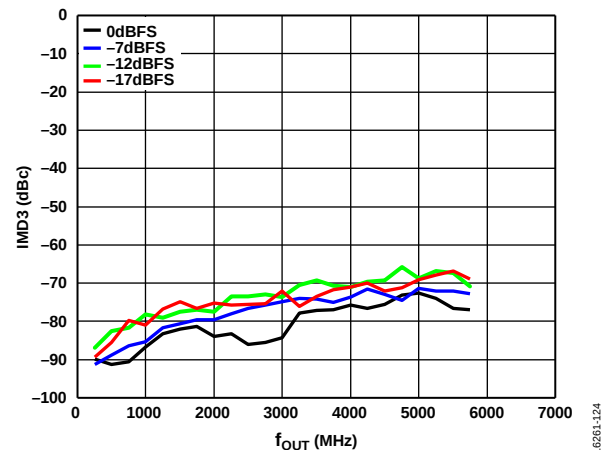
Figure 24. IMD3 vs. f_{OUT} over Digital Scale (Mode 9), 12 GHz DAC Sample Rate, Channel Interpolation 1 \times , Main Interpolation 12 \times , 1 MHz Tone Spacing
