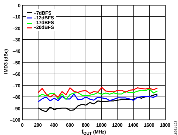
Figure 23. IMD3 vs. f_{OUT} over Digital Scale (Mode 17), 3.4 GHz DAC Sample Rate, Channel Interpolation 1 \times , Main Interpolation 1 \times , 1 MHz Tone Spacing, 11-Bit Resolution
