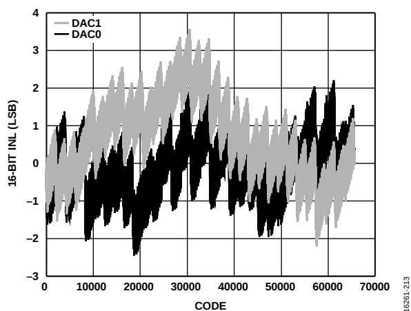
Figure 39. INL, I_{OUTFS} = 15.6 mA, 16-Bit Resolution
