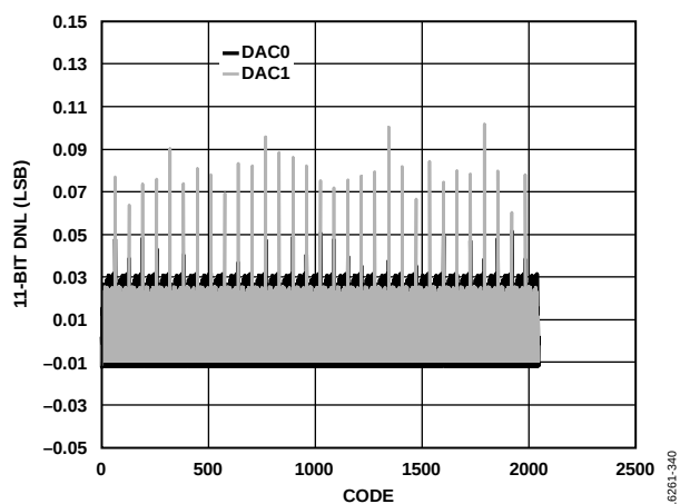
Figure 42. DNL, I_{OUTFS} = 20 mA, 11-Bit Resolution
