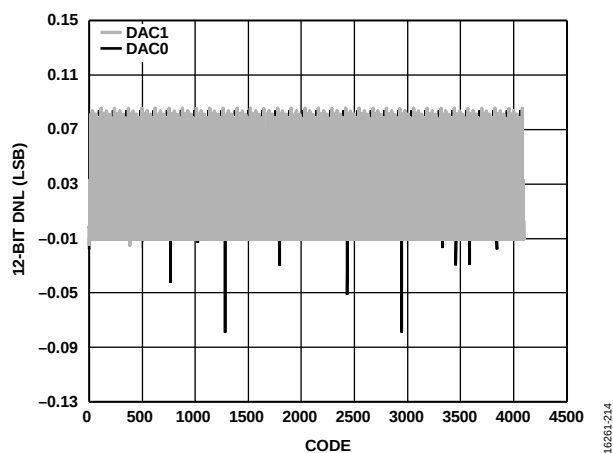
Figure 40. DNL, I_{OUTFS} = 20 mA, 12-Bit Resolution
