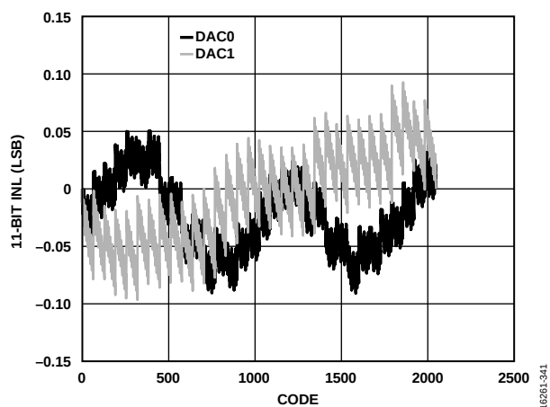
Figure 43. INL, I_{OUTFS} = 20 mA, 11-Bit Resolution
