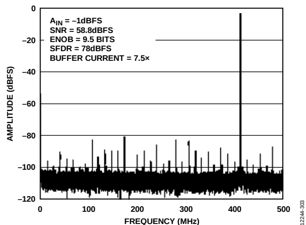
Figure 13. Single-Tone FFT with f_{IN} = 1413.3 MHz
