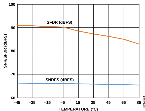
Figure 46. SNR/SFDR vs. Temperature, f_{IN} = 170.3\text{ MHz}
