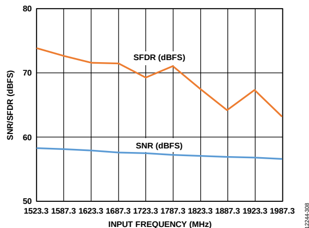
Figure 17. SNR/SFDR vs. Input Frequency; 1500 \text{ MHz} < f_{IN} < 2000 MHz; Buffer Current = 8.5\times (Uses Circuit Shown in Figure 64)
