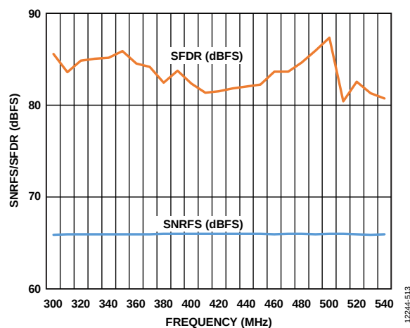
Figure 37. SNR/SFDR vs. Sample Rate ( f_s ), f_{IN} = 170.3 MHz; Buffer Current = 3.0\times
