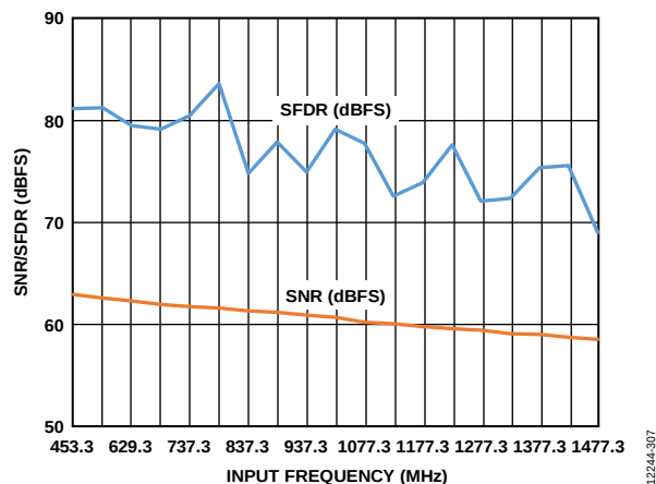
Figure 16. SNR/SFDR vs. Input Frequency; 450 \text{ MHz} < f_{IN} < 1500 MHz; Buffer Current = 7.5\times (Uses Circuit Shown in Figure 64)
