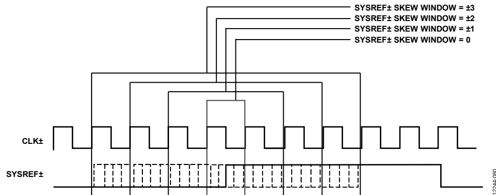
Figure 113. SYSREF_{\pm} Skew Window
