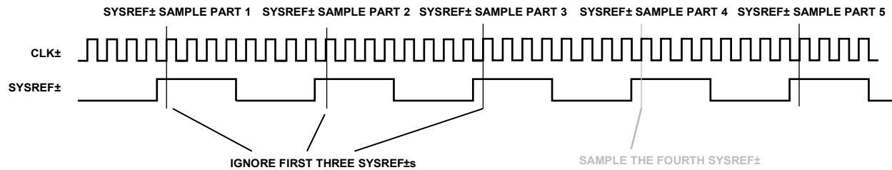
Figure 112. SYSREF_{\pm} Ignore Example; SYSREF_{\pm} Ignore Count Bits (Register 0x121, Bits[3:0]) = 3
