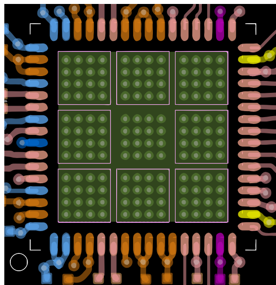
Figure 118. Recommended PCB Layout of Exposed Pad for the AD9234
