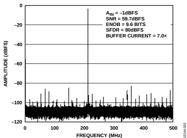
Figure 12. Single-Tone FFT with f_{IN} = 1213.3 MHz
