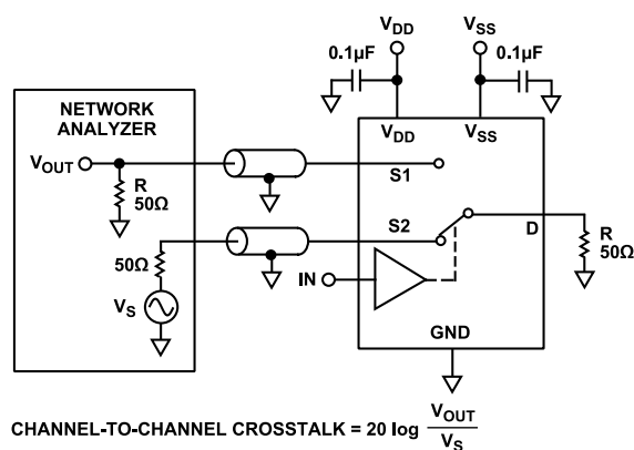
Figure 22. Channel-to-Channel Crosstalk
