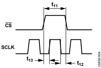
Figure 4. SCLK/ \overline{\text{CS}} Timing Diagram
