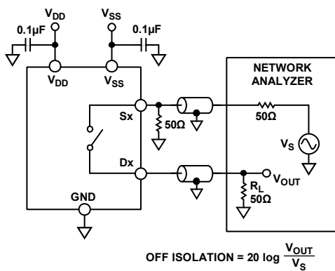
Figure 26. Off Isolation
