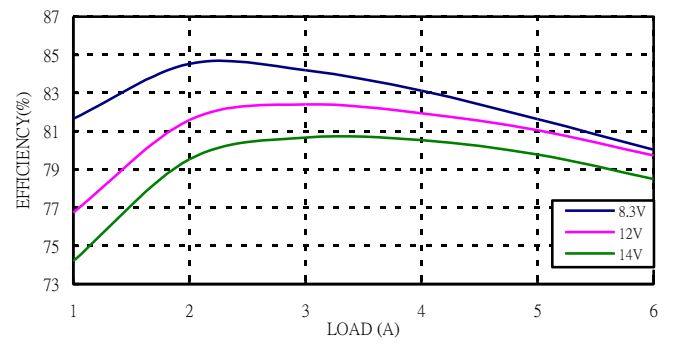
Figure 2: Converter efficiency vs. output current (1.2V output voltage)
