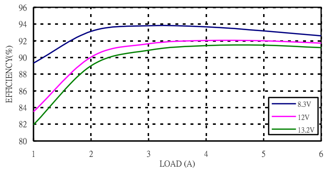
Figure 7: Converter efficiency vs. output current (5.0V output voltage)
