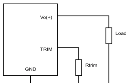
Figure 23: Circuit configuration for programming output voltage using an external resistor
