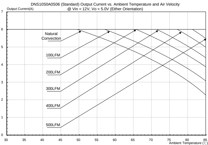
Figure 32: DNS10S0A0S06(Standard) Output current vs. ambient temperature and air velocity@ Vin=12V, Vo=5.0V (Either Orientation)
