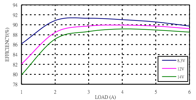
Figure 4: Converter efficiency vs. output current (1.8V output voltage)
