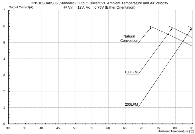
Figure 34: DNS10S0A0S06(Standard) Output current vs. ambient temperature and air velocity@ Vin=12V, Vo=0.75V (Either Orientation)
