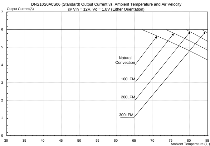
Figure 33: DNS10S0A0S06(Standard) Output current vs. ambient temperature and air velocity@ Vin=12V, Vo=1.8V (Either Orientation)
