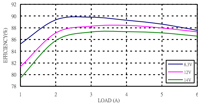
Figure 3: Converter efficiency vs. output current (1.5V output voltage)
