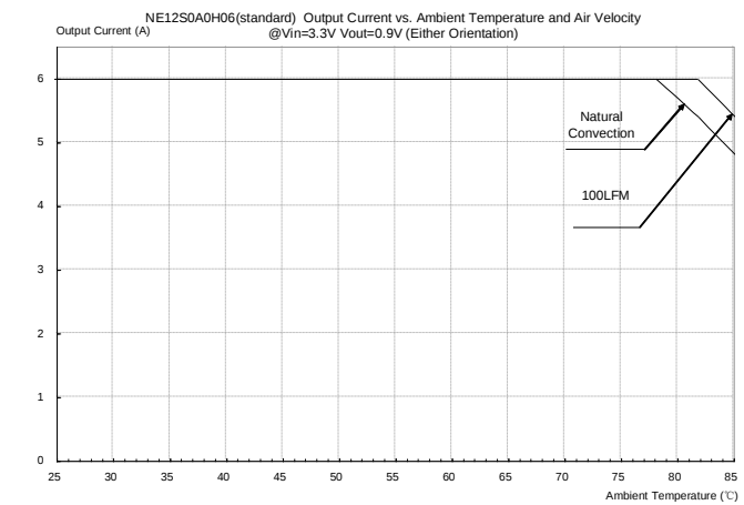
Figure 40: Output current vs. ambient temperature and air velocity @Vin=3.3V, Vout=0.9V (Either Orientation)
