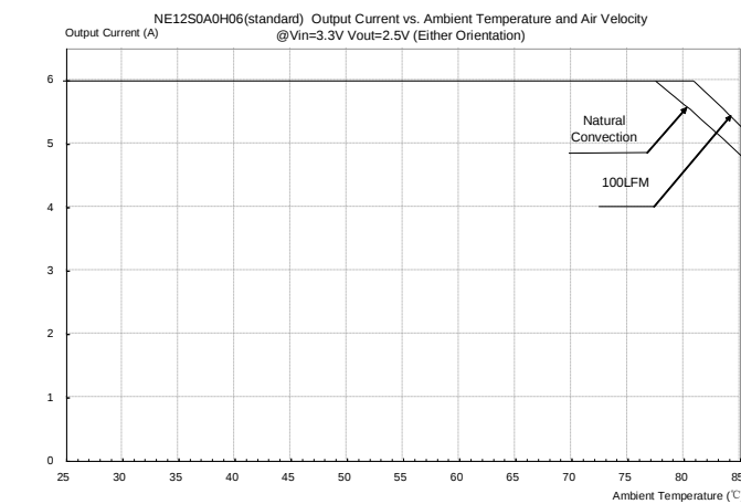
Figure 41: Output current vs. ambient temperature and air velocity @ Vin =3.3V, Vout=2.5V (Either Orientation)
