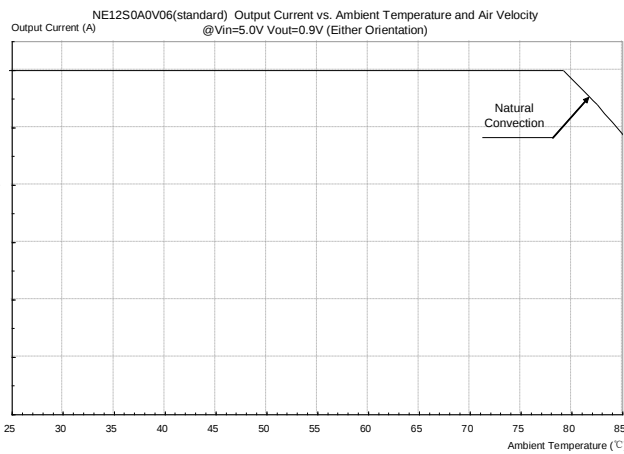
Figure 30: Output current vs. ambient temperature and air velocity @ Vin =5V, Vout=0.9V (Either Orientation)
