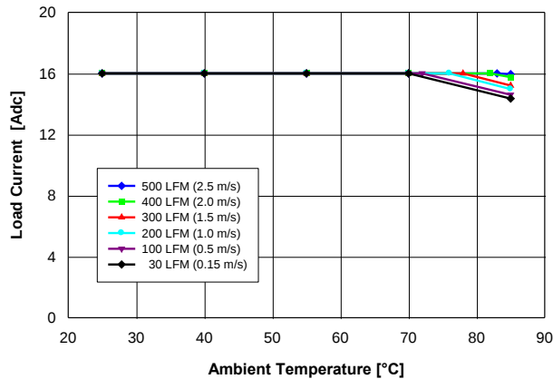
Fig. 2.0V.1: Available load current vs. ambient temperature and airflow rates for V_{out} = 2.0V converter mounted vertically with V_{in} = 12V , and maximum MOSFET temperature \leq 120^{\circ}C .
