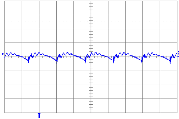
Fig. 1.0V.5: Output voltage ripple (20mV/div.) at full rated load current into a resistive load with external capacitance 100μF ceramic + 1μF ceramic and V_{in} = 12V for V_{out} = 1.0V . Time scale: 2μs/div.
