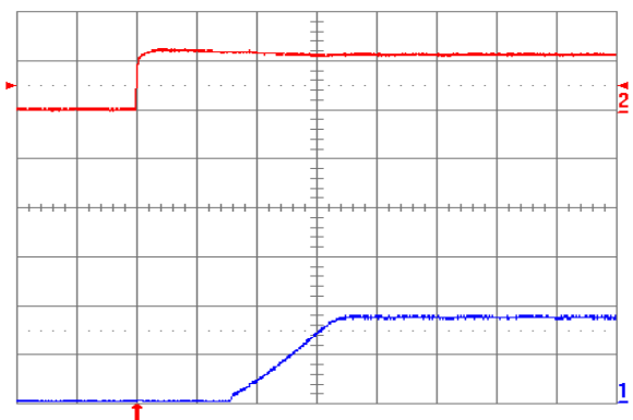
Fig. 1.8V.4: Turn-on transient for V_{out} = 1.8V with application of V_{in} at full rated load current (resistive) and 100 \mu F external capacitance at V_{in} = 12V . Top trace: V_{in} (10V/div.); Bottom trace: output voltage (1V/div.); Time scale: 2ms/div.
