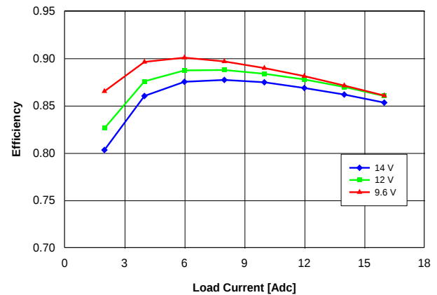
Fig. 1.5V.2: Efficiency vs. load current and input voltage for V_{out} = 1.5V converter mounted vertically with air flowing at a rate of 200 LFM (1 m/s) and T_a = 25 ^{\circ}\text{C} .
