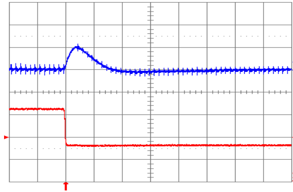
Fig. 1.2V.7: Output voltage response for V_{out} = 1.2V to negative load current step change from 16A to 8A with slew rate of -5A/\mu s at V_{in} = 12V . Top trace: output voltage (200mV/div.); Bottom trace: load current (5A/div.). C_o = 100\mu F ceramic. Time scale: 20 \mu s /div.
