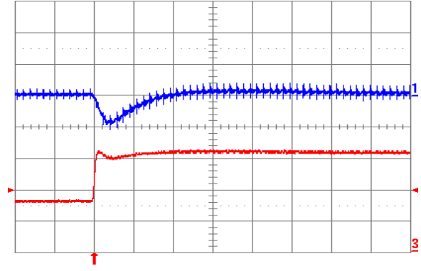
Fig. 1.0V.6: Output voltage response for V_{out} = 1.0V to positive load current step change from 8A to 16A with slew rate of 5A/μs at V_{in} = 12V . Top trace: output voltage (200mV/div.); Bottom trace: load current (5A/div.). C_o = 100μF ceramic. Time scale: 20μs/div.
