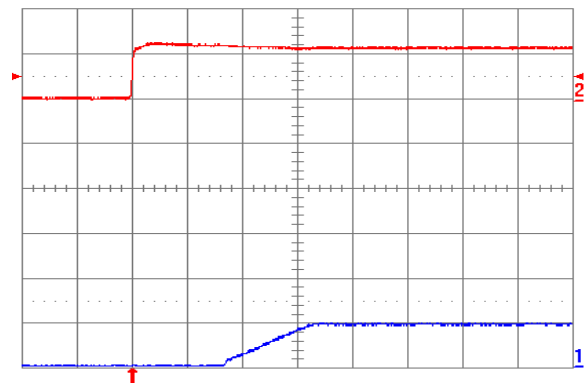
Fig. 1.0V.4: Turn-on transient for V_{out} = 1.0V with application of V_{in} at full rated load current (resistive) and 100 \mu F external capacitance at V_{in} = 12V . Top trace: V_{in} (10V/div.); Bottom trace: output voltage (1V/div.); Time scale: 2ms/div.
