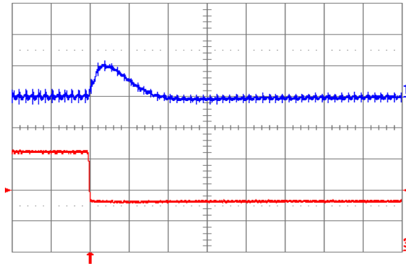
Fig. 2.0V.7: Output voltage response for V_{out} = 2.0V to negative load current step change from 16A to 8A with slew rate of -5A/\mu s at V_{in} = 12V . Top trace: output voltage (200mV/div.); Bottom trace: load current (5A/div.). C_o = 100\mu F ceramic. Time scale: 20 \mu s /div.
