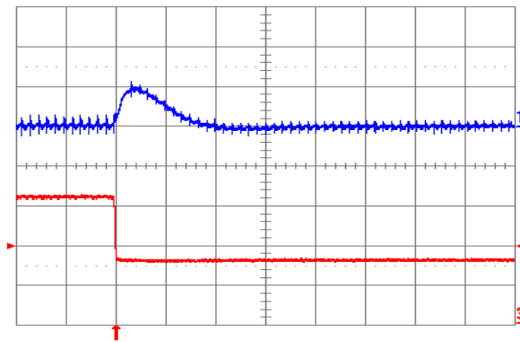
Fig. 1.8V.7: Output voltage response for V_{out} = 1.8V to negative load current step change from 16A to 8A with slew rate of -5A/ \mu s at V_{in} = 12V. Top trace: output voltage (200mV/div.); Bottom trace: load current (5A/div.). C_o = 100 \mu F ceramic. Time scale: 20 \mu s/div.
