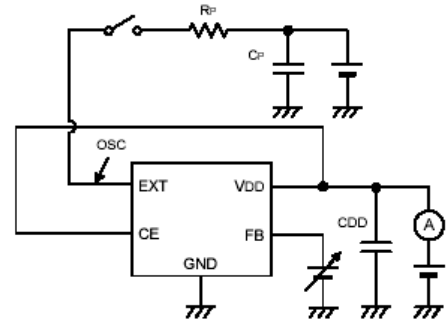
Circuit ④
