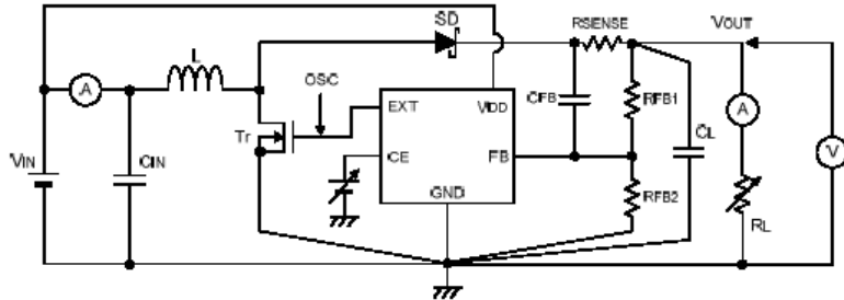
Circuit ①
