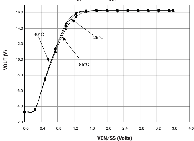
Output Voltage vs. EN/SS Voltage vs. Temperature, V_{IN} = 3.6V ; V_{OUT} = 16V
