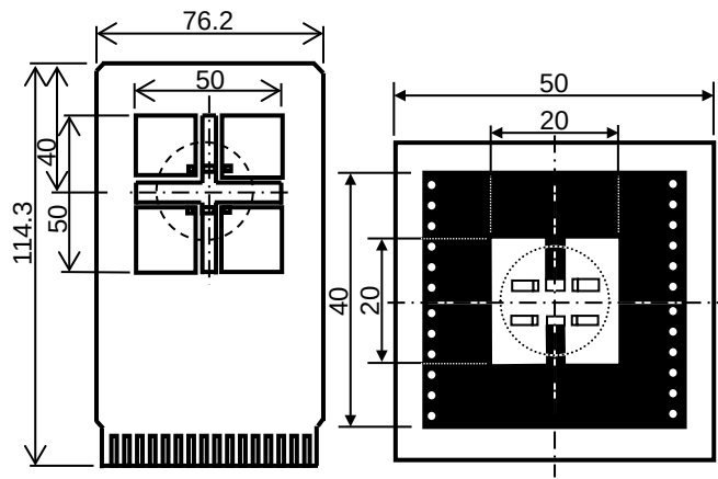
○ IC Mount Area (mm)
