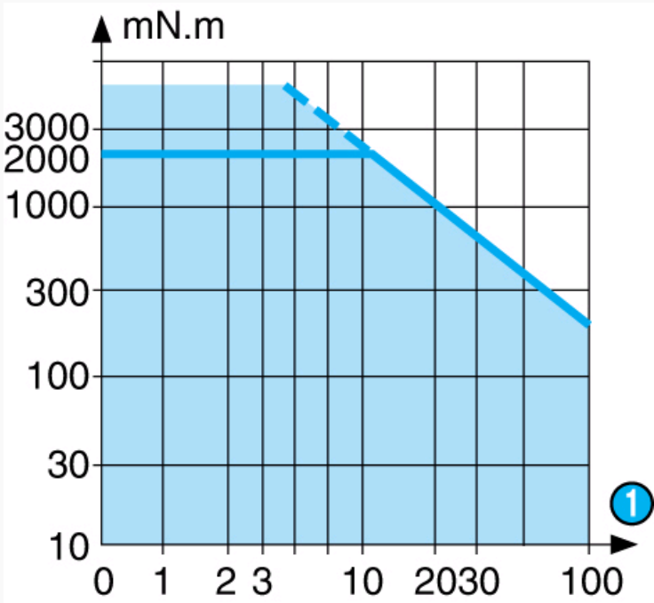
Curve : torque/nominal speed
