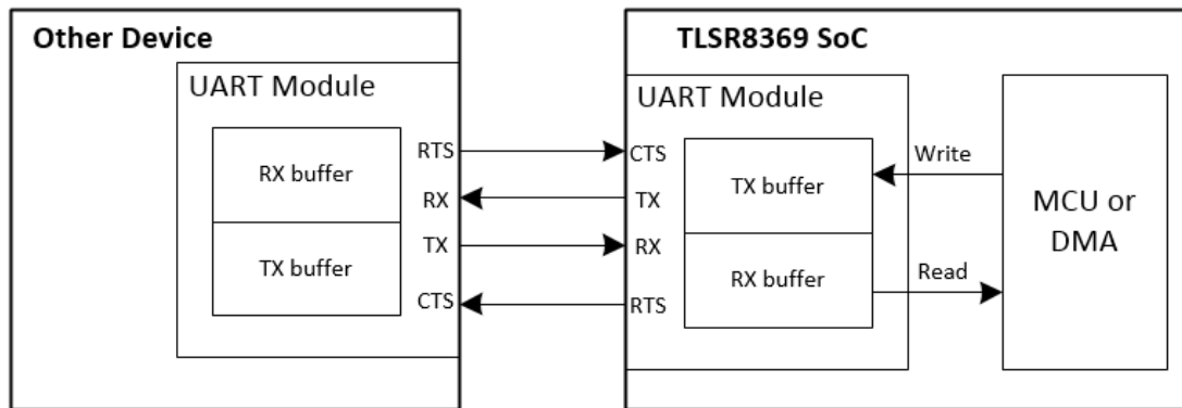
Figure 7- 9 UART communication
