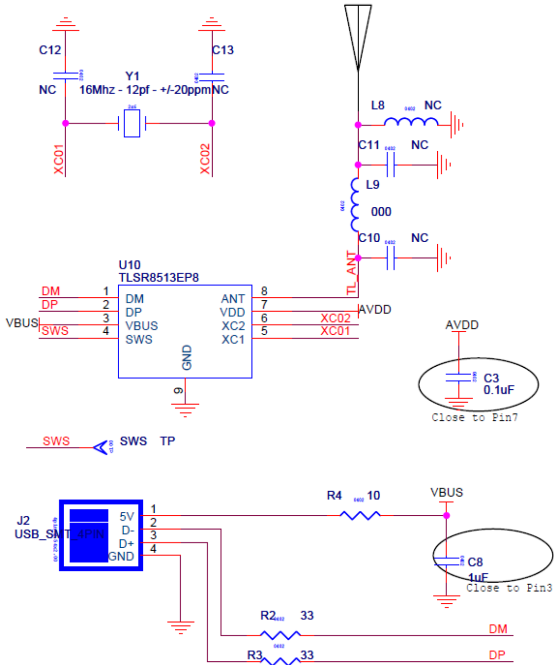
Figure 7- 3 Schematic for TLSR8513EP8
