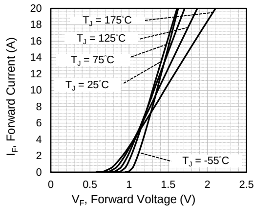
Fig.1 Forward Characteristics
