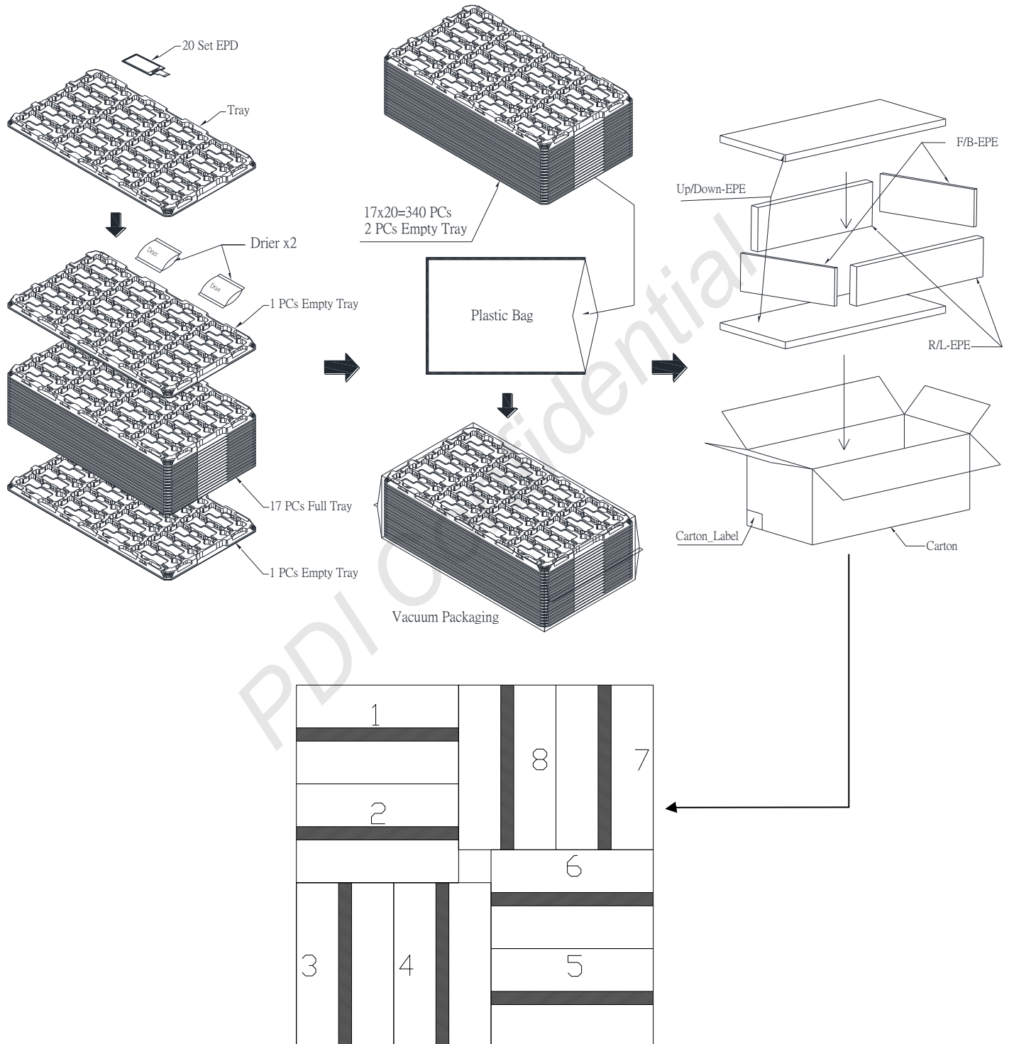
Figure 7-1 Packing Diagram
