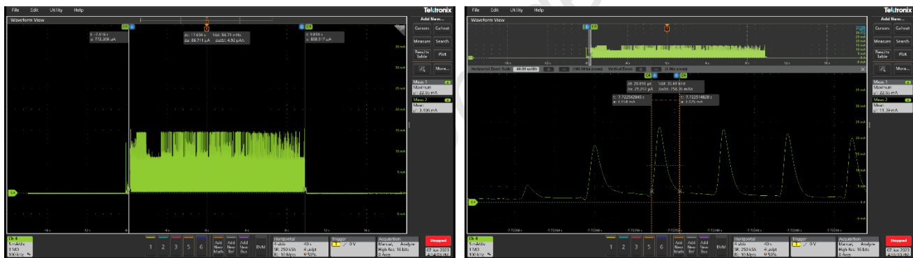
Figure 3-2 Image Update Current Profile
