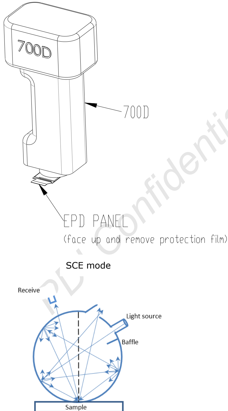
Figure 6-1 Optical measurement
