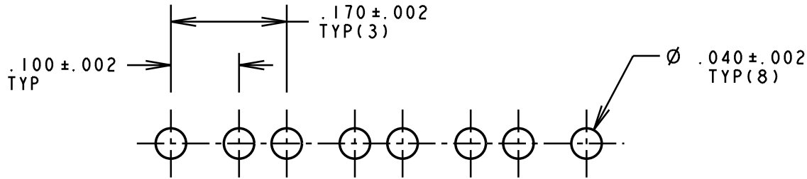
RECOMMENDED PC BOARD HOLE PATTERN
