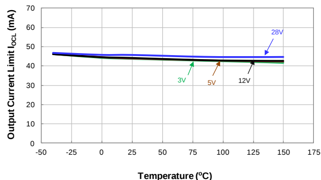
Output Current Limit vs Temperature
