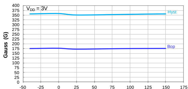
Temperature ( ^\circ\text{C} ) Switch Operate Point B_{op} vs Temperature
