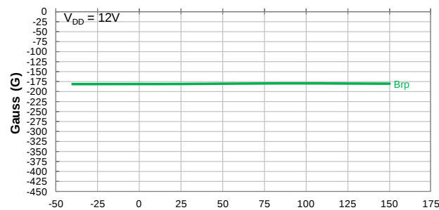
Temperature ( ^\circ\text{C} ) Switch Release Point B_{rp} vs Temperature
