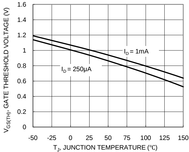
Figure 15. Q1 Gate Threshold Variation vs. Junction Temperature
