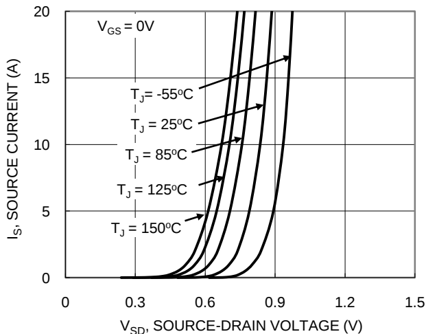
Figure 17. Q1 Diode Forward Voltage vs. Current
