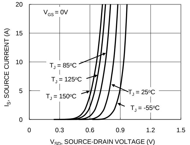
Figure 18. Q2 Diode Forward Voltage vs. Current
