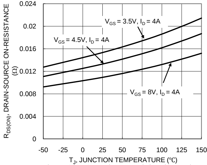
Figure 13. Q1 On-Resistance Variation with Junction Temperature
