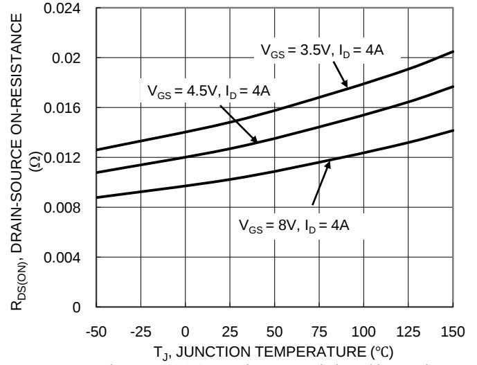
Figure 14. Q2 On-Resistance Variation with Junction Temperature
