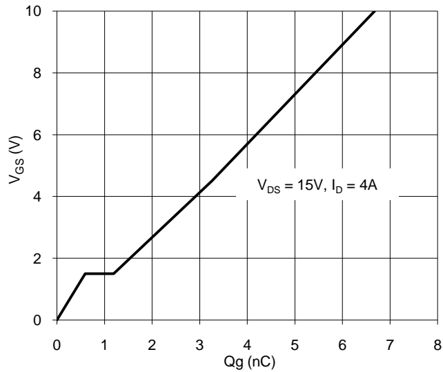
Figure 21. Gate Charge
