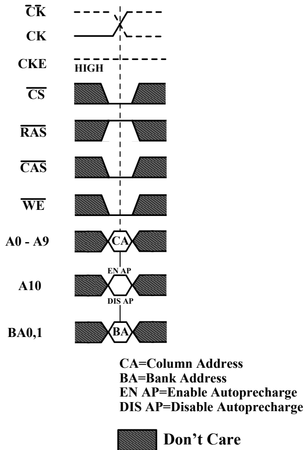
Figure 16. Write Command
