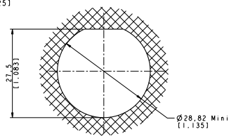
Panel Drilling
