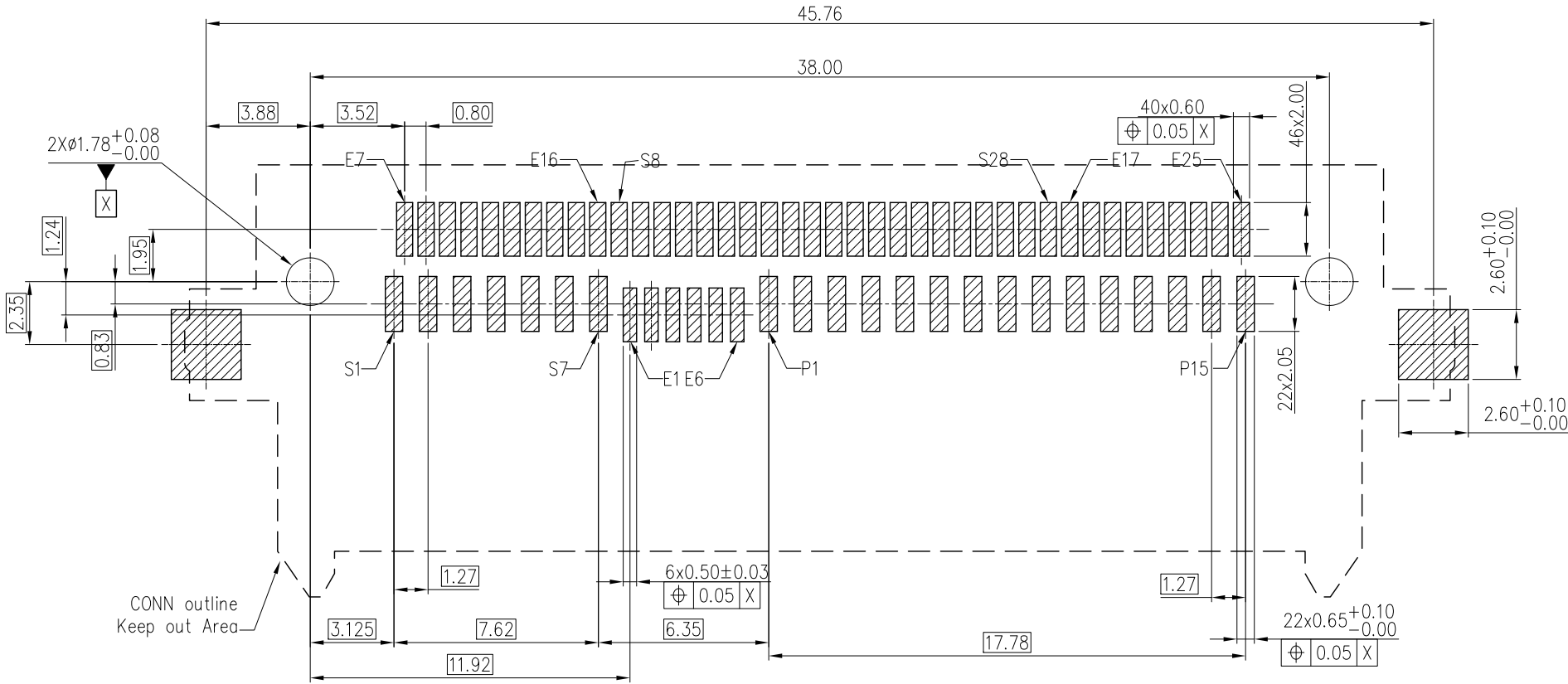
RECOMMENDED PCB LAYOUT GENERAL TOLERANCE ±0.05mm
