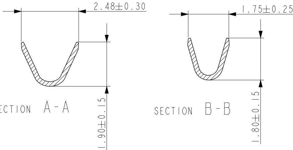
CROSS SECTIONS FOR CT #20-24
