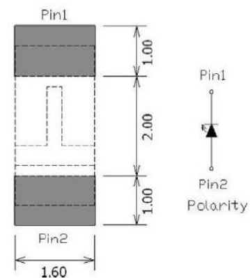
Figure 1. IN-S126ETHIR Solder Pattern
