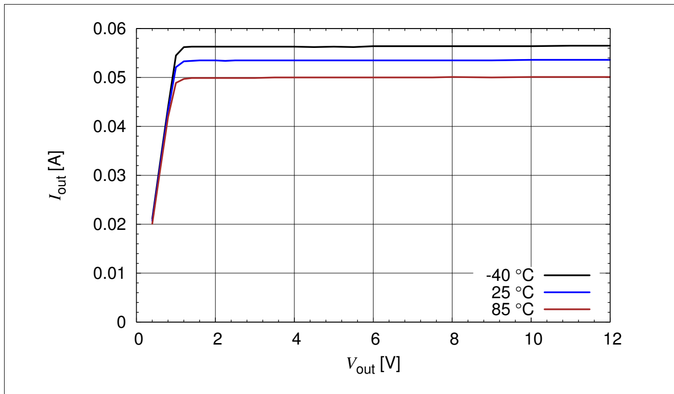
Figure 3-17 BCR 421U: Output Current versus V_{out} I_{out} = f(V_{out}) , V_{EN} = 3.3 V, R_{ext} = 20 Ω, T_A = \text{Parameter}
