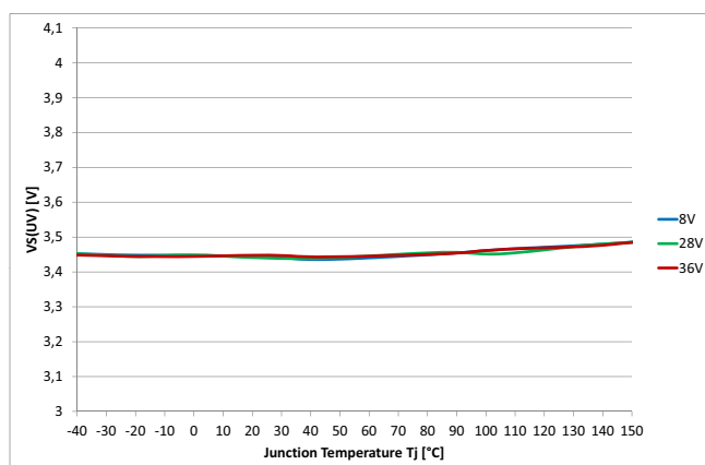
Figure 41 Switch OFF Energy E_{OFF} = f(T_J; V_S) , R_L = 12 \Omega
