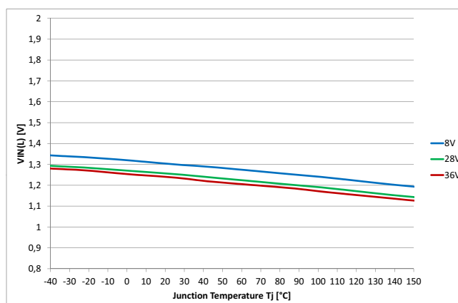
Figure 48 Input Voltage Threshold V_{IN(L)} = f(T_J; V_S)
