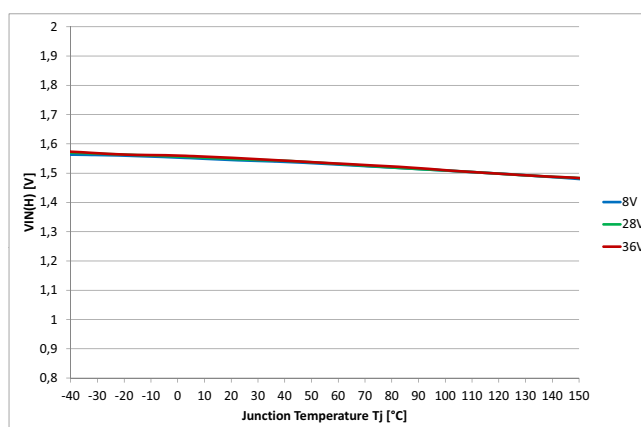
Figure 49 Input Voltage Threshold V_{IN(H)} = f(T_J; V_S)
