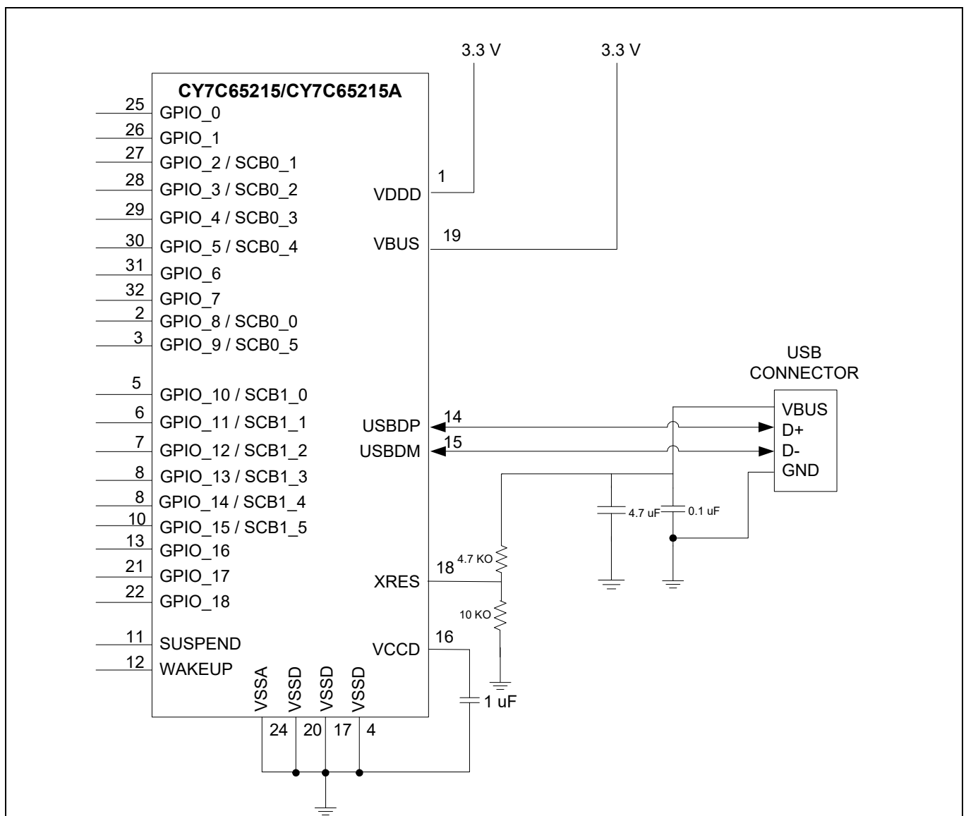
Figure 5 Self-powered configuration
