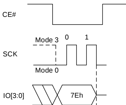
Figure 8.138 Gang Sector/Block Lock Sequence In QPI Mode
