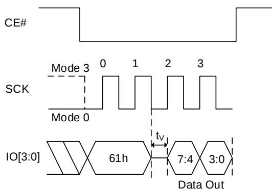
Figure 8.65 Read Read Parameters Sequence In QPI Mode
