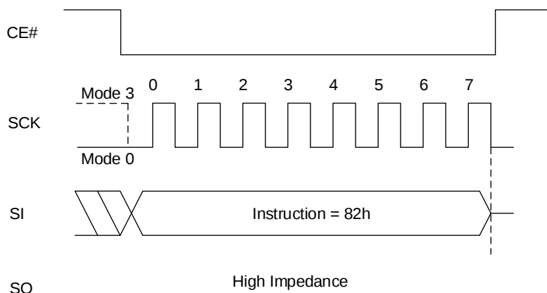
Figure 8.46 Clear Extended Read Register Sequence In SPI Mode
