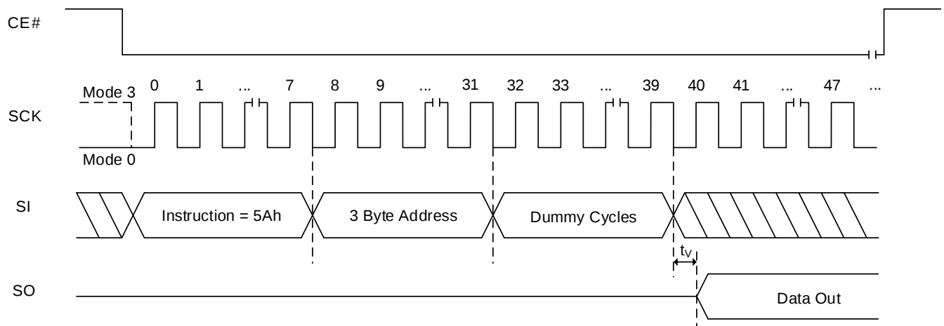
Figure 8.55 RDSFDP (Read SFDP) Sequence
